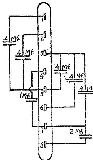
INTERNAL CONNECTIONS OF FILTER CONDENSERS
